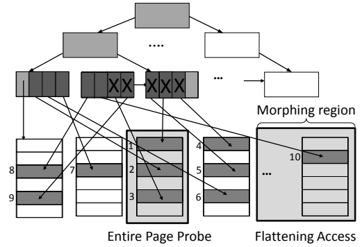
Fig. 7: Smooth Scan access pattern.
