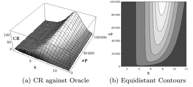
Fig. 11: The CR of Selectivity Increase Smooth Scan when compared against Oracle.
