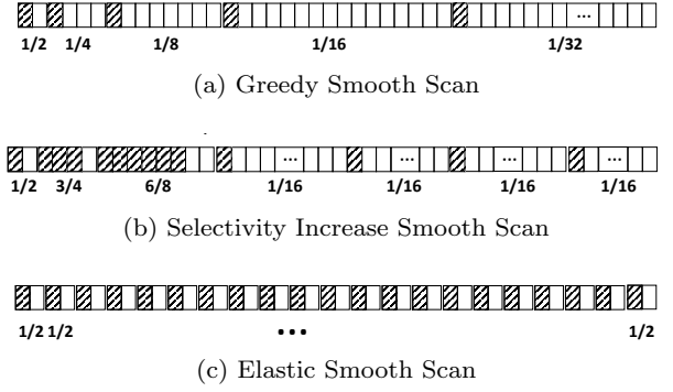
Fig. 8: Worst case result distributions for Smooth Scan alternatives.
