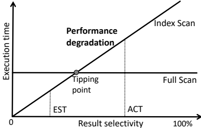
Fig. 2: Access path selection sensitivity to cardinality estimation.
