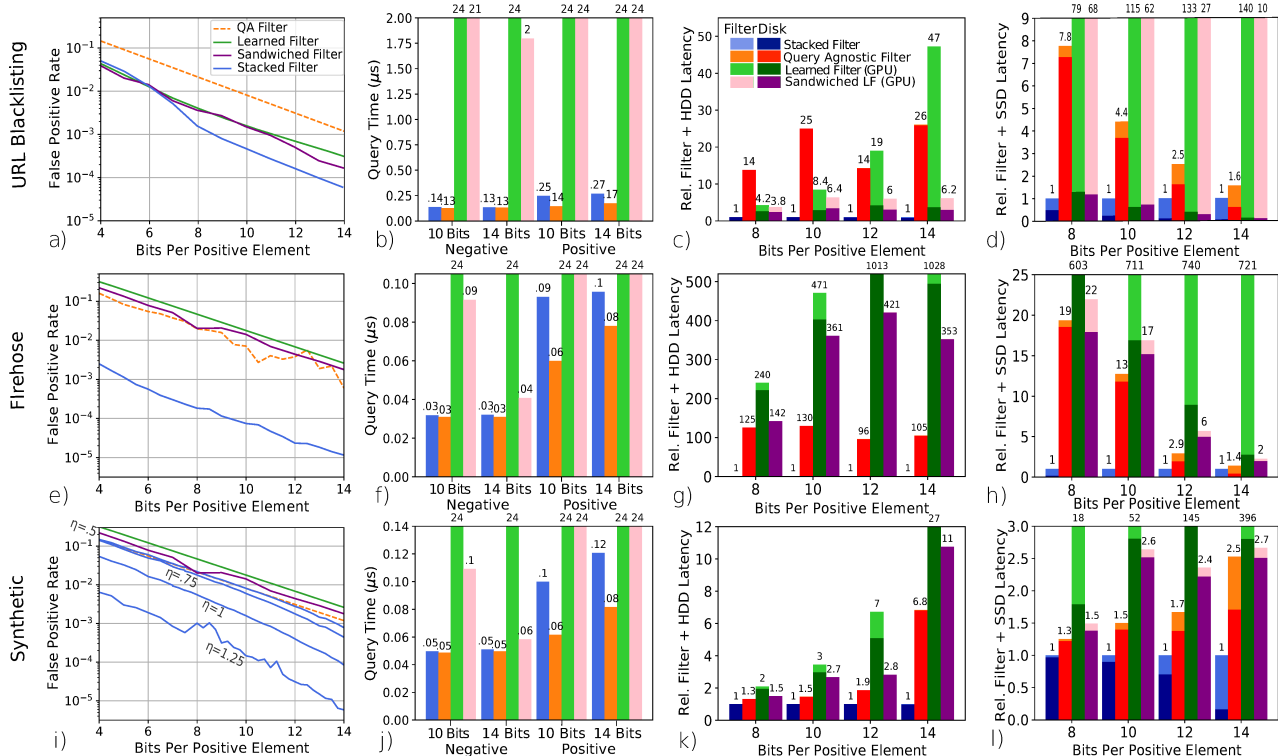
Figure 3: Stacked Bloom Filters achieve a similar EFPR to Learned Bloom Filters while maintaining a 170x throughput advantage and beat both query-agnostic and learned filters in overall performance on typical workloads.
